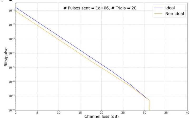
Figure 1: Bits/pulse VS. Channel loss of an ideal a non-ideal stochastic simulation of the MDI-QKD protocol. Imperfections include polarization and arrival times mismatch, fluctuations of laser frequency; efficiency and jitter of the detectors, and dark and solar counts. These flaws decrease the number of key bits generated with the same number of pulses sent, thus decreasing the key rate. The simulation allows to evaluate the impact of the different defects with respect to an ideal transmission scenario.
