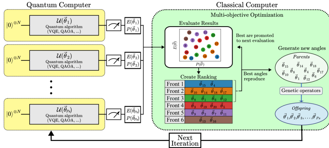
Figure 1 – Schematic diagram of the constrained multi-objective variational optimizer (MOVCO).
