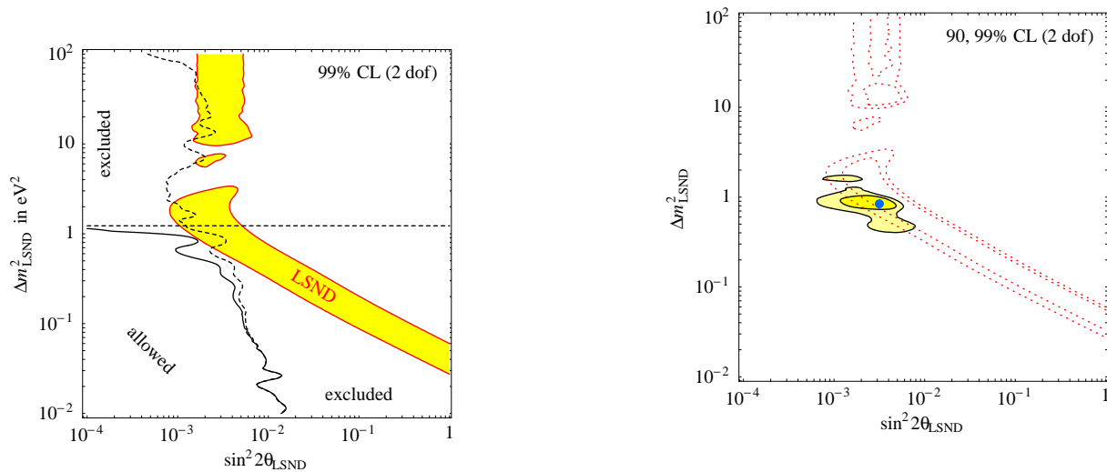
Figure 9: Best fit , all data ; 3 + 1 sterile \nu solution (CPT cons.) disfavoured by WMAP since (\Delta m_{LSND}^2)^{1/2} \simeq \sum m_\nu .
